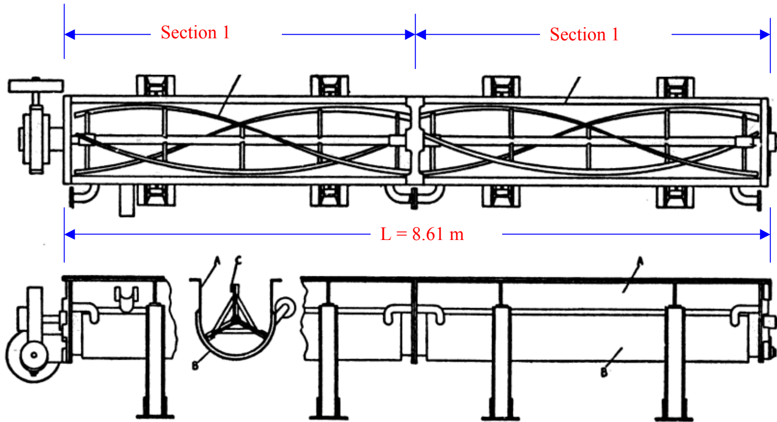
FIG. 11-2. Swenson-Walker crystallizer: A, trough; B, jackets; C, agitator.
